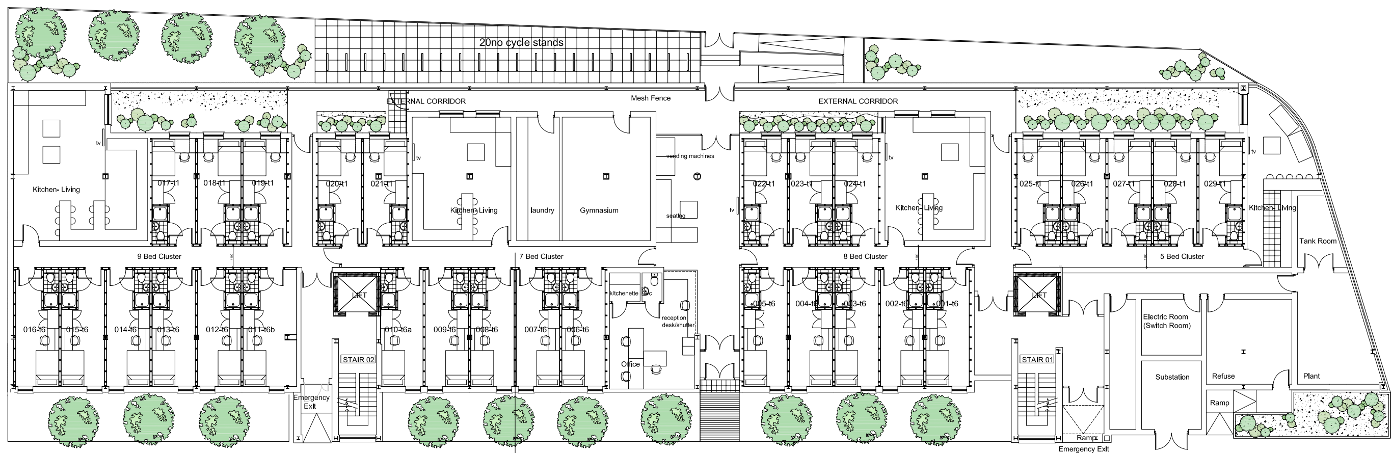
GROUND FLOOR
